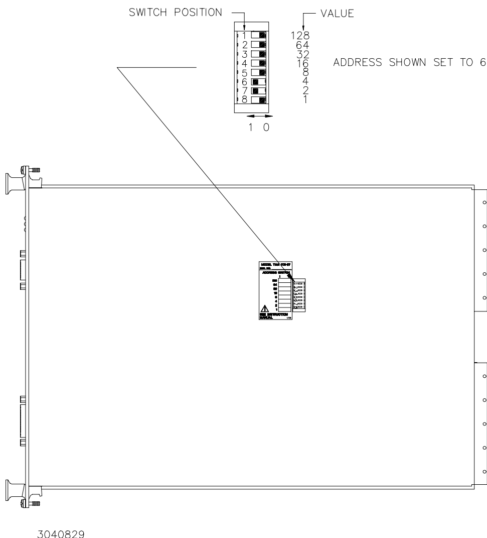
FIGURE 2-1. VXI ADDRESS SELECT
