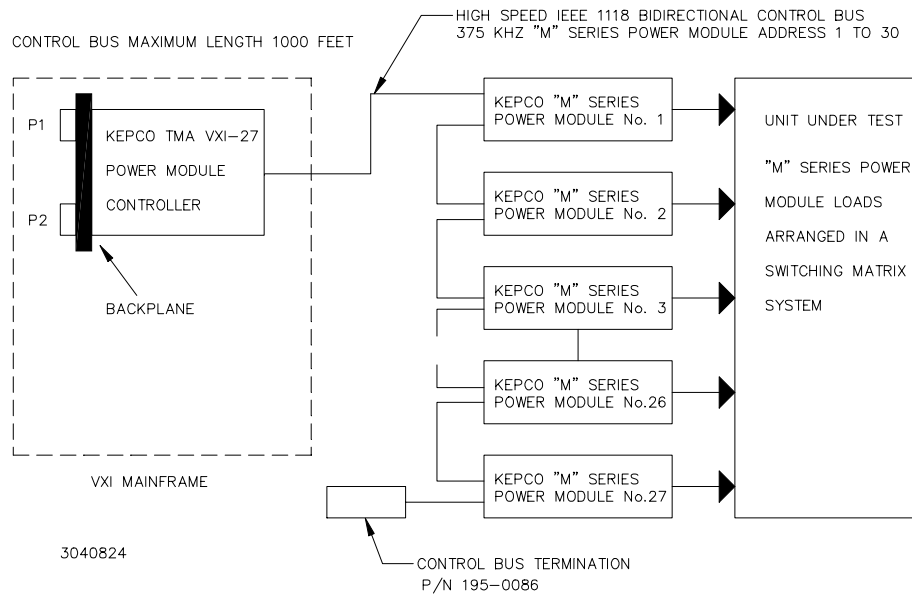
FIGURE 1-2. TYPICAL CONTROLLER TO POWER MODULE INTERFACE
