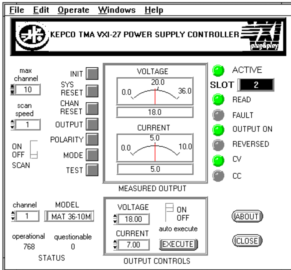
FIGURE 3-3. TMA VXI-27 plug&play PANEL
