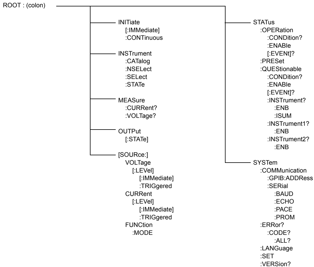
FIGURE 3-4. TREE DIAGRAM OF SCPI COMMANDS USED WITH TMA VXI-27 CONTROLLER
